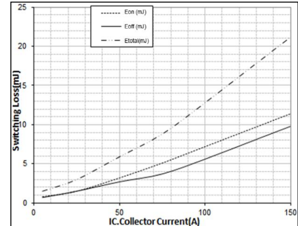
Inverter IGBT Switching Loss vs. IC T_{vj}=25^{\circ}\text{C} , V_{GE}=15\text{V} , V_{CE}=600\text{V} , R_g=13\Omega
