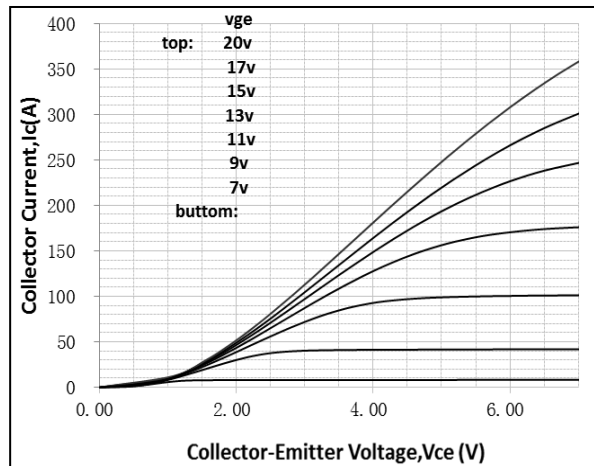
Inverter IGBT output characteristic I_C = f(V_{CE}) ( T_{vj}=150^{\circ}\text{C} )
