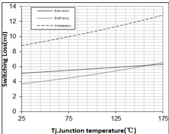
Inverter IGBT Switching Loss vs. Tvj V_{GE}=15\text{V} , V_{CE}=600\text{V} , I_C=75\text{A}
