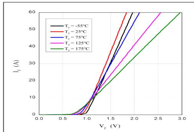
Diode Characteristic
