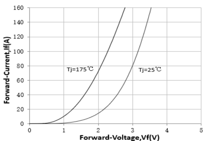
Diode Characteristic
