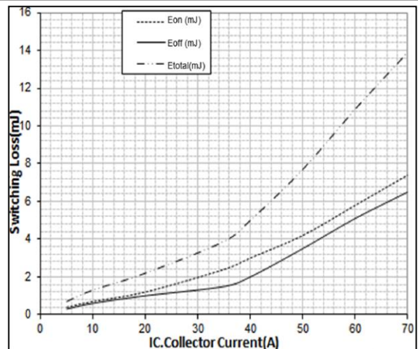
Inverter IGBT Switching Loss vs. IC
