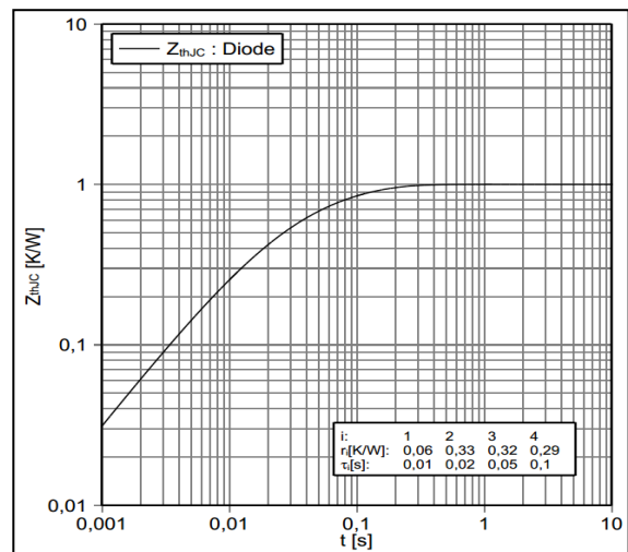
Inverter FRD Transient Thermal Impedance
