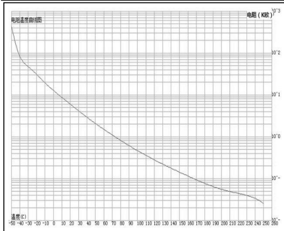
NTC-Thermistor-temperature characteristic(typical)
