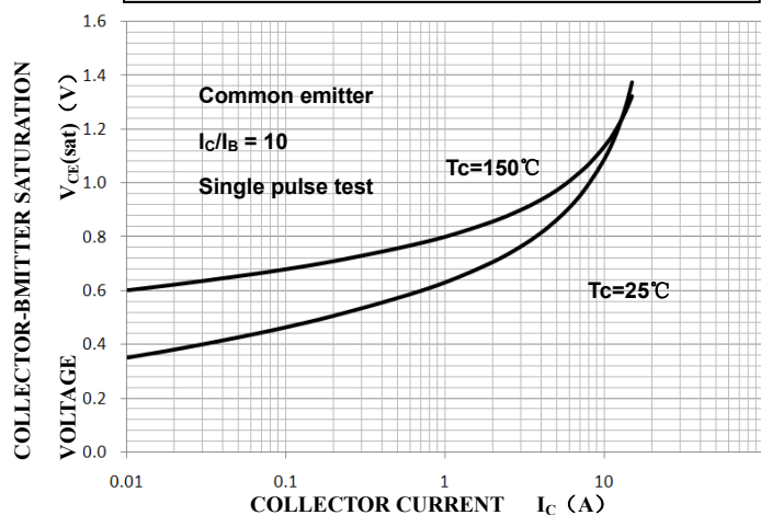
Saturation Voltage
