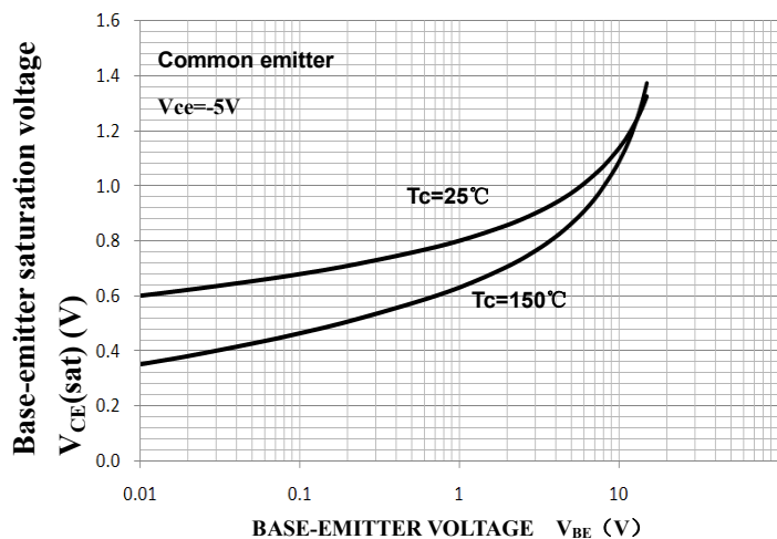
Base-Emitter Voltage
