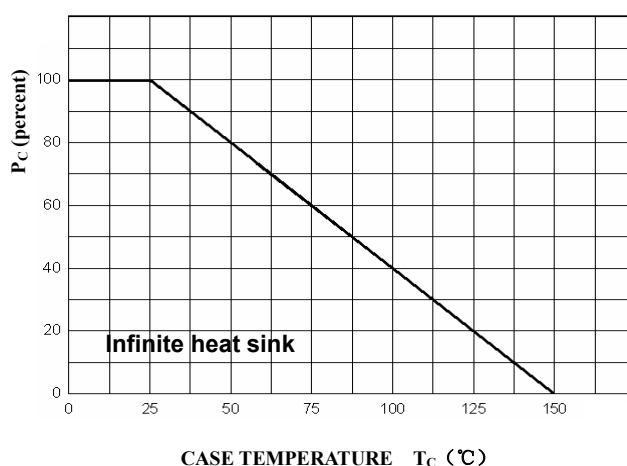
Power Derating
