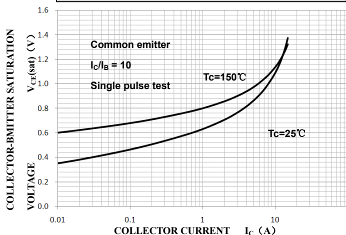
Saturation Voltage
