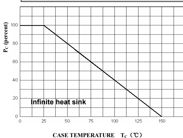
Power Derating
