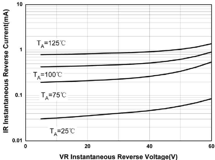
I_R vs V_R
