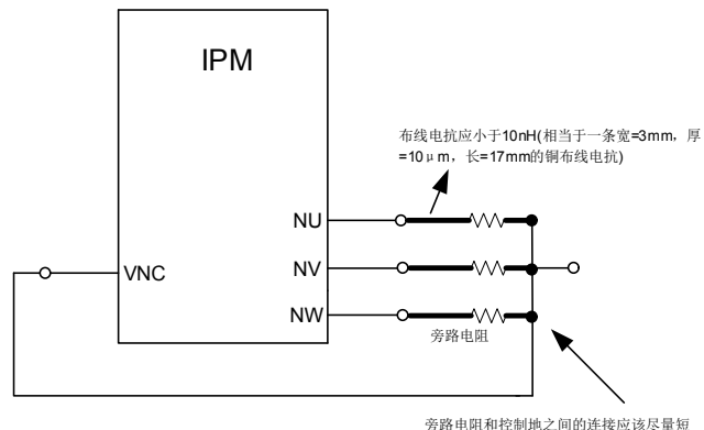
图 14: 旁路电阻接线注意事项 Fig 14: Recommended Wiring Around The Shunt Resisto
