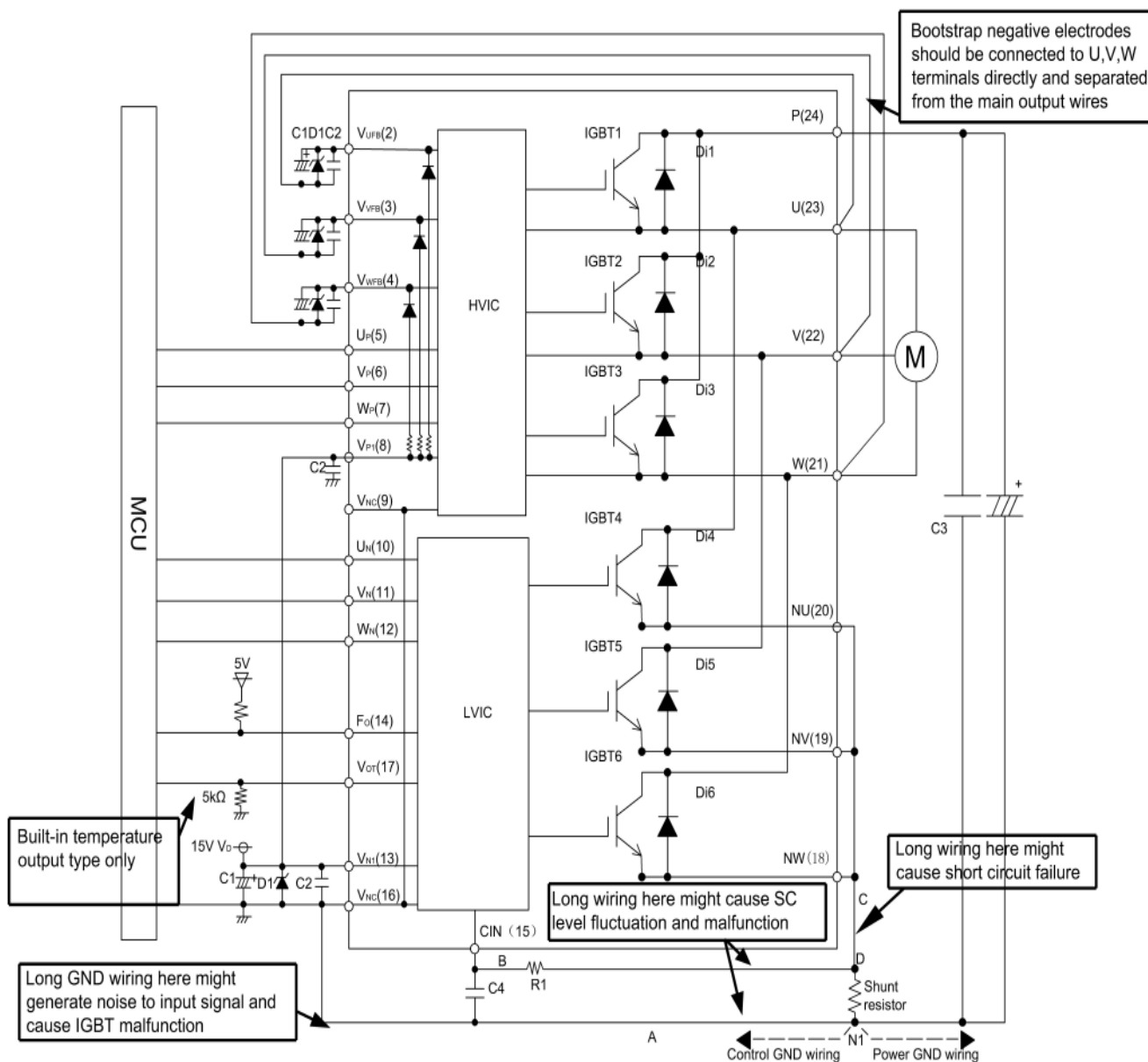
典型应用电路图 Typical application circuit diagram
