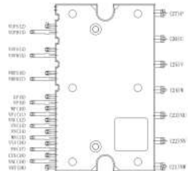
DIP28-DBC
