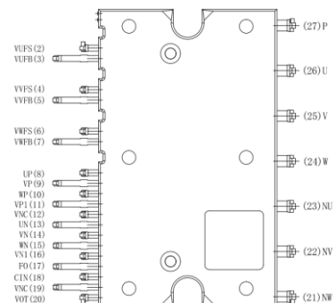
DIP28-DBC
