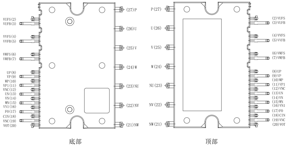
Fig 1: Internal circuit
