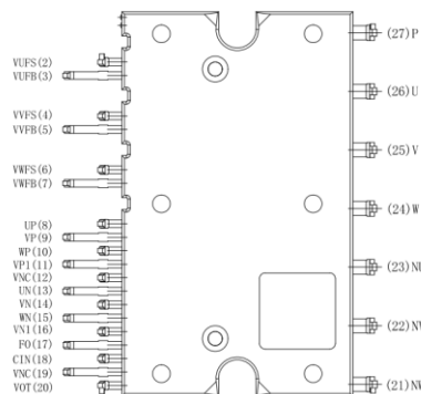
DIP28-DBC
