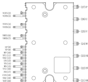
DIP28-DBC
