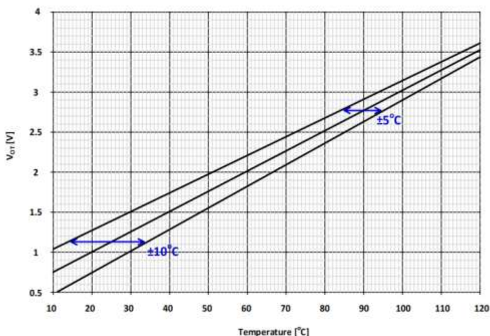
图 6.1: VOT 输出电压曲线 Figure 6.1: VOT output voltage curve
