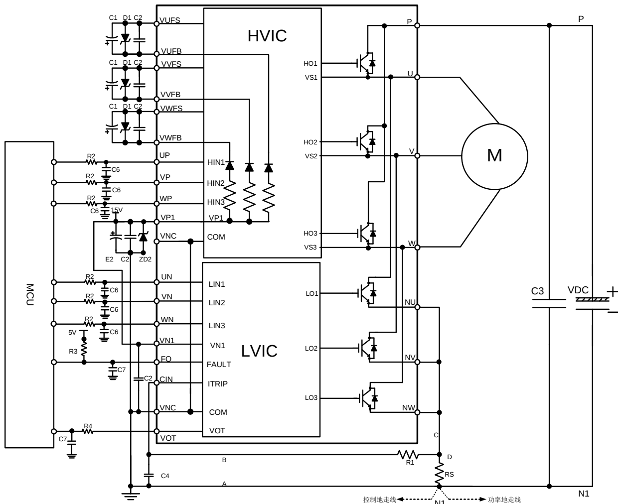
典型应用电路图 Typical application circuit diagram
