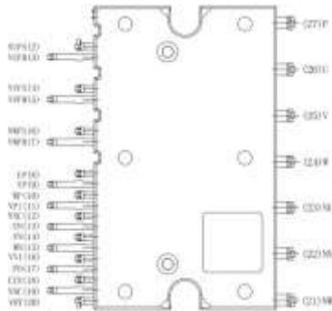
DIP28-DBC
