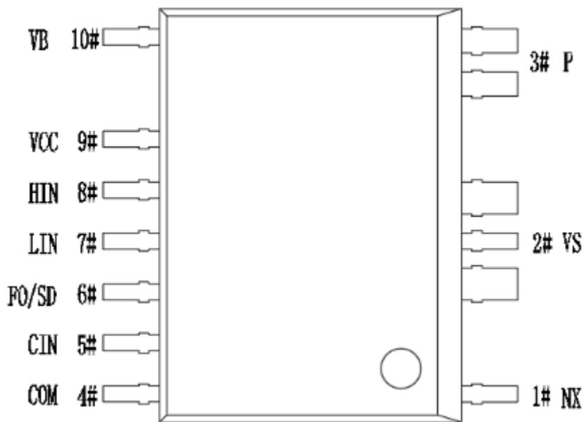
Fig 1: Internal circuit
