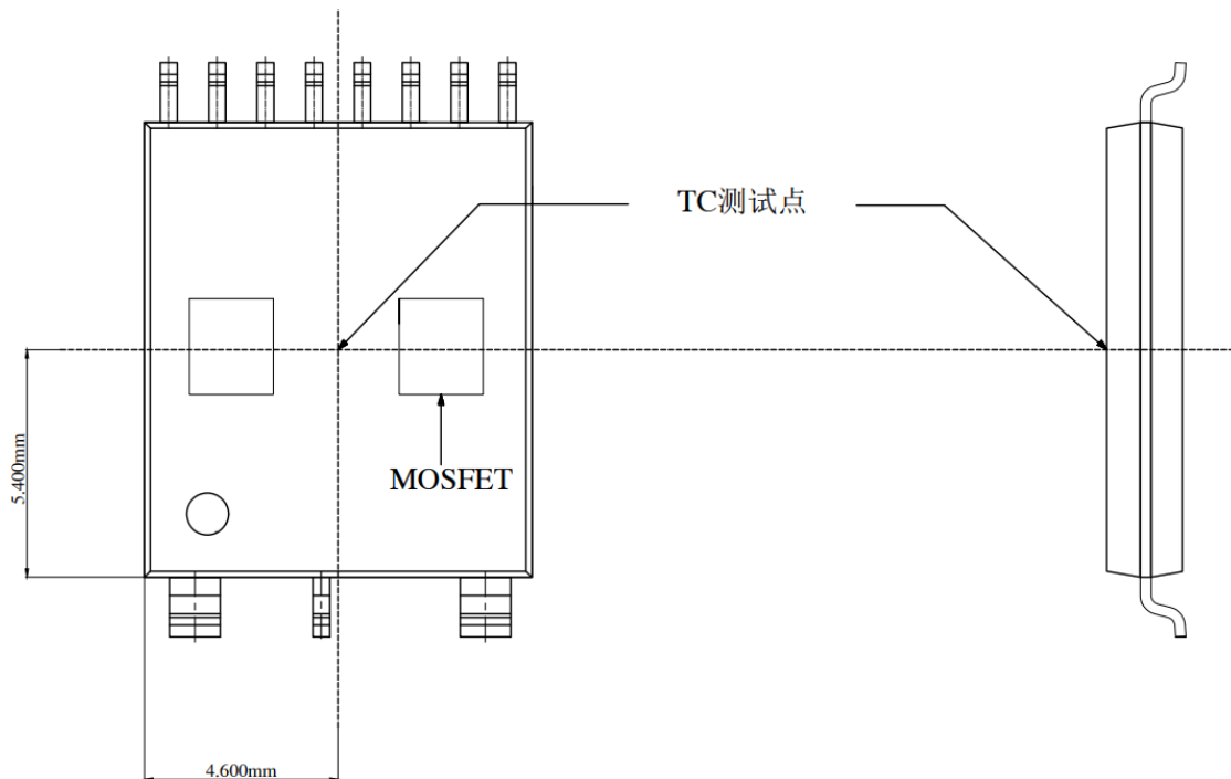
图 6: 壳温 T_c 测试点 Fig 6: Case Temperature Measurement
