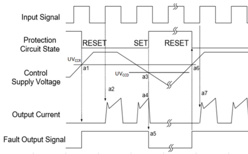
图 7: 欠压保护时序图(低侧) Fig 7: Undervoltage protection sequence diagram (low side)
