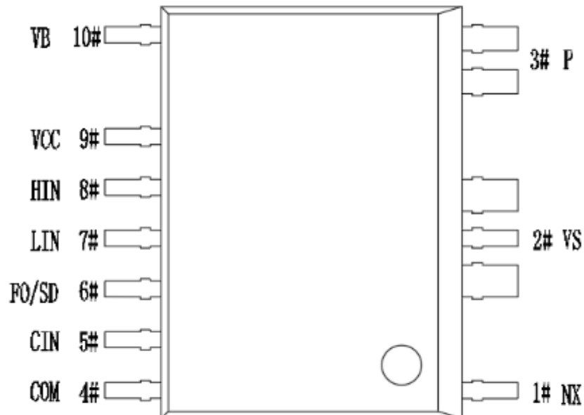
Fig 1: Internal circuit
