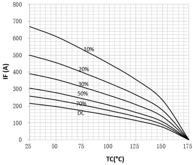
Current Derating
