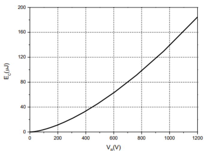
Capacitance Stored EnergyFigure
