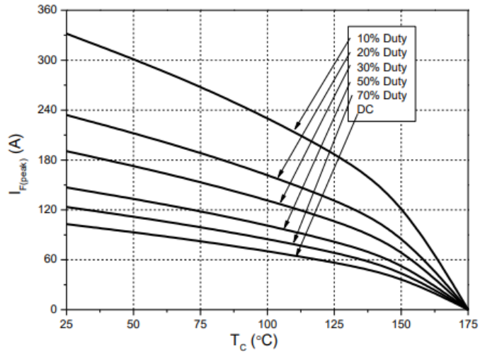
Current Derating
