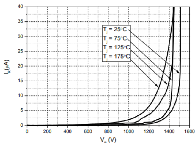
Reverse Characteristics
