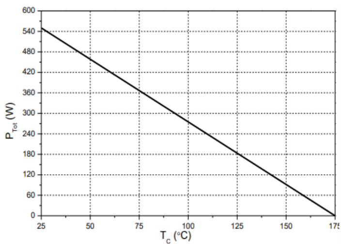
Power Derating
