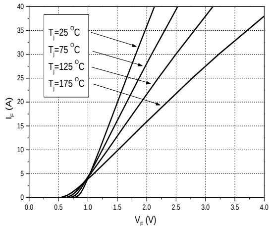
Figure 1. Forward Characteristics
