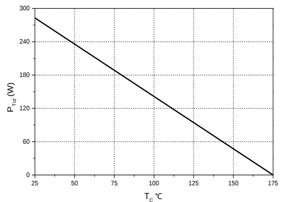
Figure 6. Power Derating
