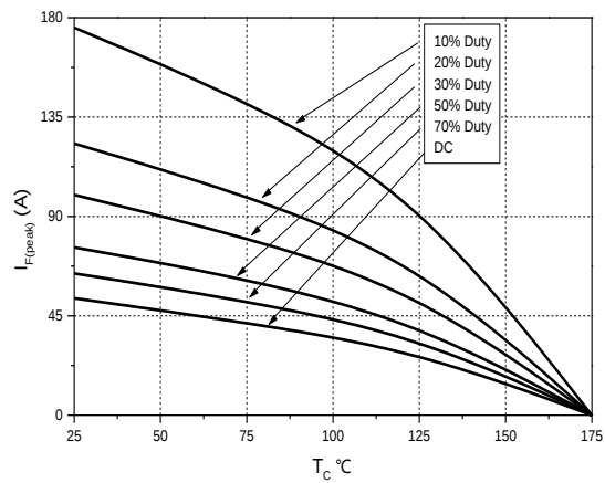
Figure 7. Current Derating
