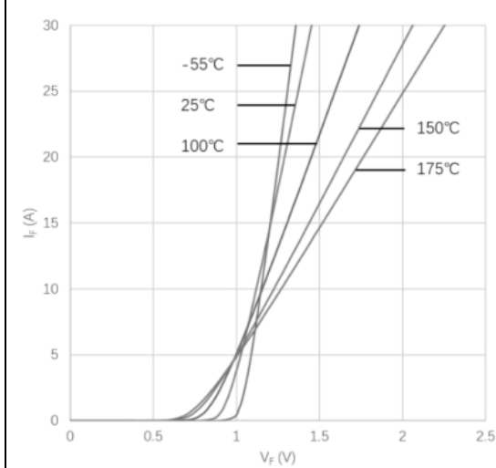
Forward Characteristics
