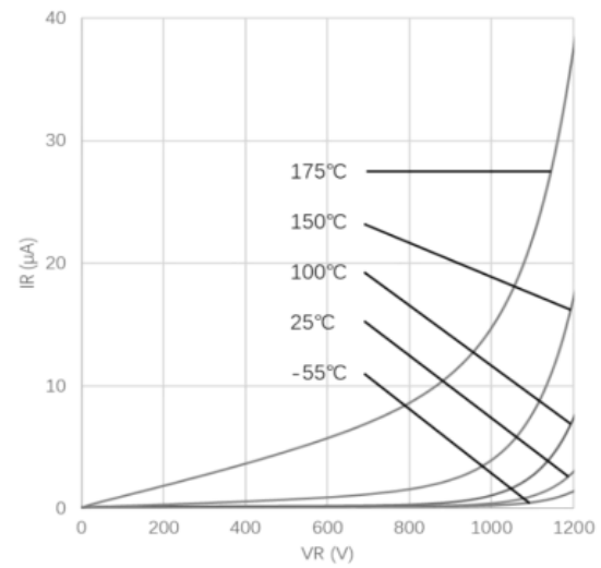
Reverse Characteristics
