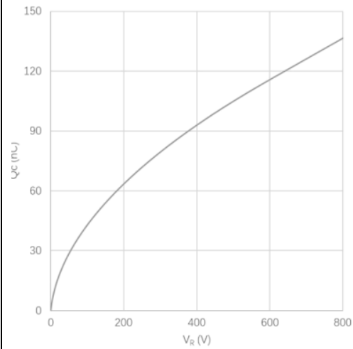
Capacitance Charge vs. Reverse Voltage
