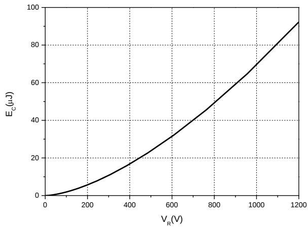
Figure 5. Capacitance Stored Energy
