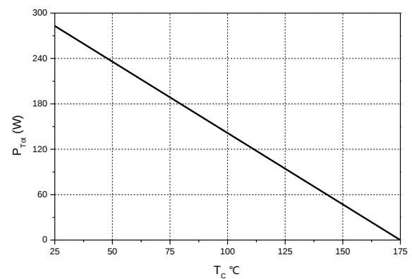
Figure 6. Power Derating
