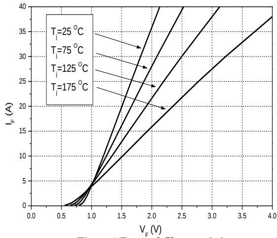
Figure 1. Forward Characteristics
