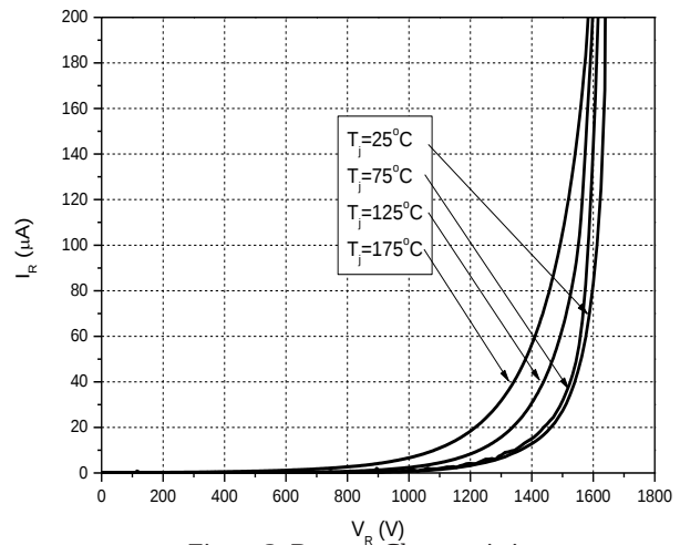
Figure 2. Reverse Characteristics
