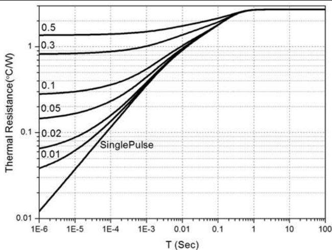
Transient Thermal Impedance (TO-3PF, TO220MF2L-K1)
