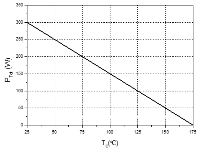
Power Derating (TO-220C-2L)
