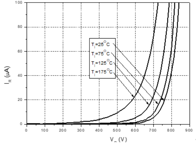
Reverse Characteristics
