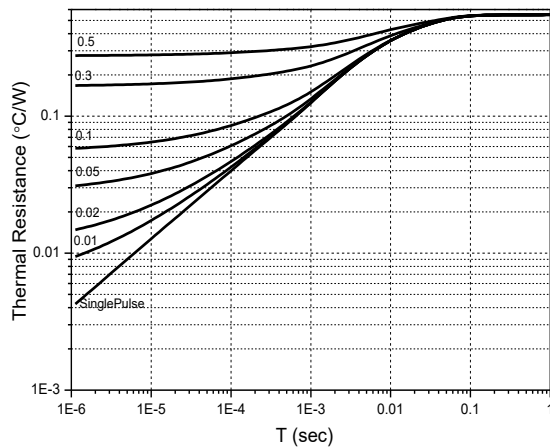
Figure 9. Transient Thermal Impedance(TO-247)
