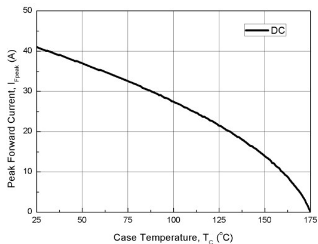
I_{Fpeak} vs T_C
