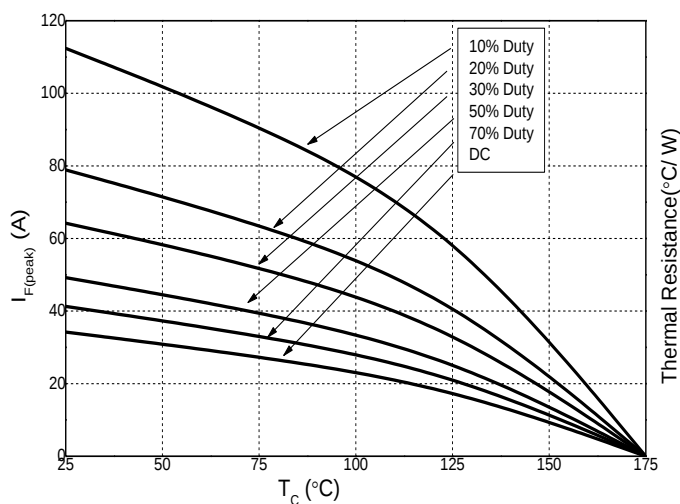
Figure 7. Current Derating
