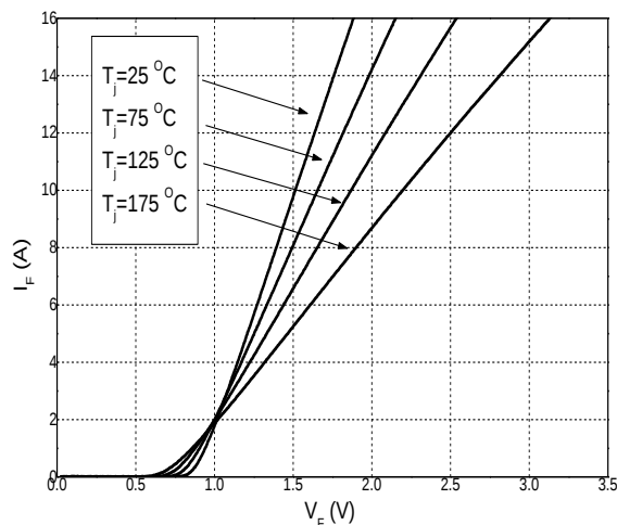
Figure 1. Forward Characteristics
