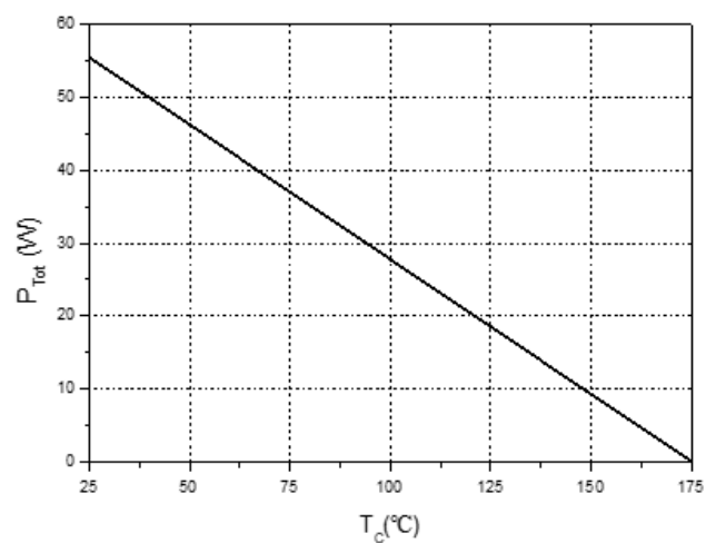
Power Derating (TO-220MF-2L)
