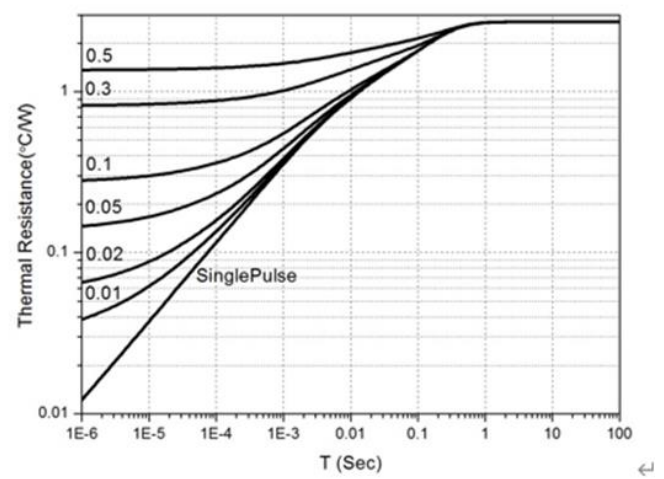
Transient Thermal Impedance (TO-220MF-2L)
