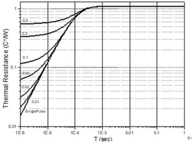
Transient Thermal Impedance (TO-220C-2L)
