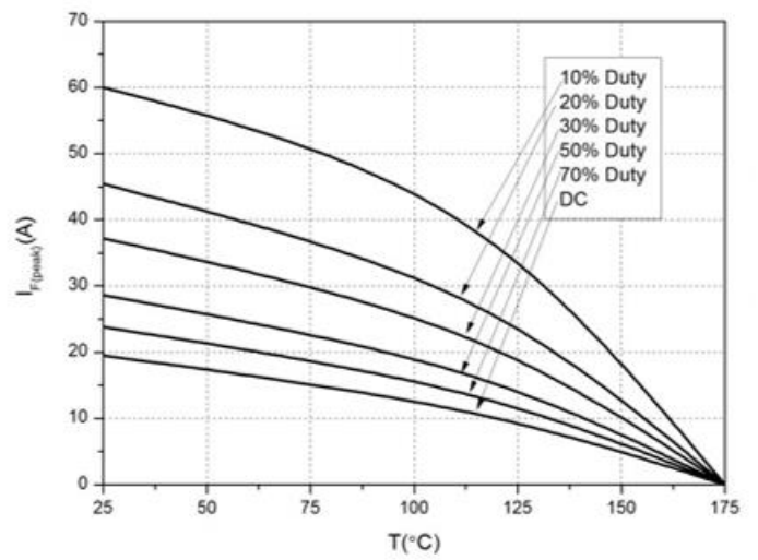
Current Derating (TO-220MF-2L)
