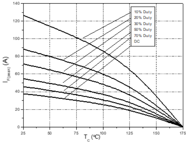
Current Derating (TO-220C-2L)
