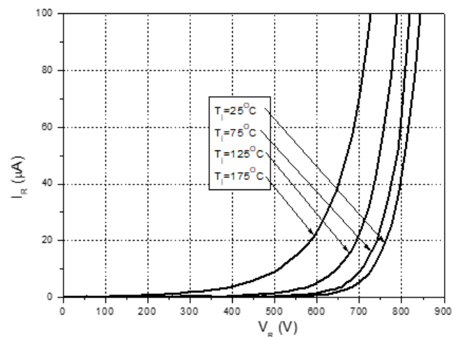
Reverse Characteristics
