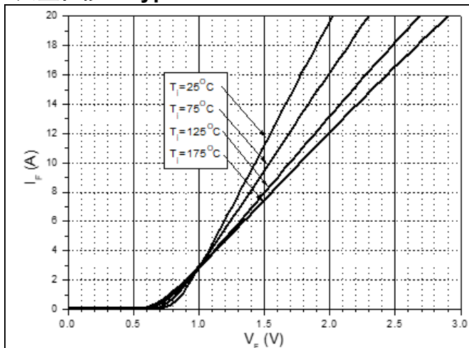
Forward Characteristics
