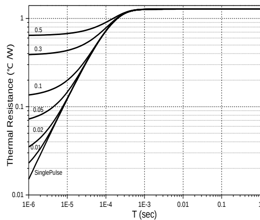
Figure 8. Transient Thermal Impedance(TO-220)
