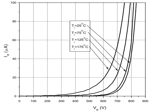
Figure 2. Reverse Characteristics
