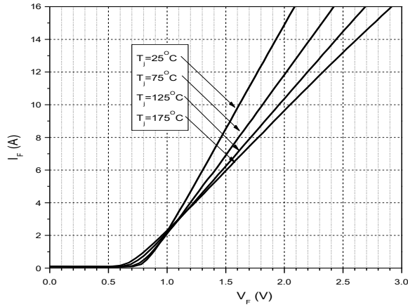
Figure 1. Forward Characteristics
