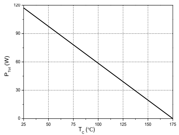
Figure 6. Power Derating
