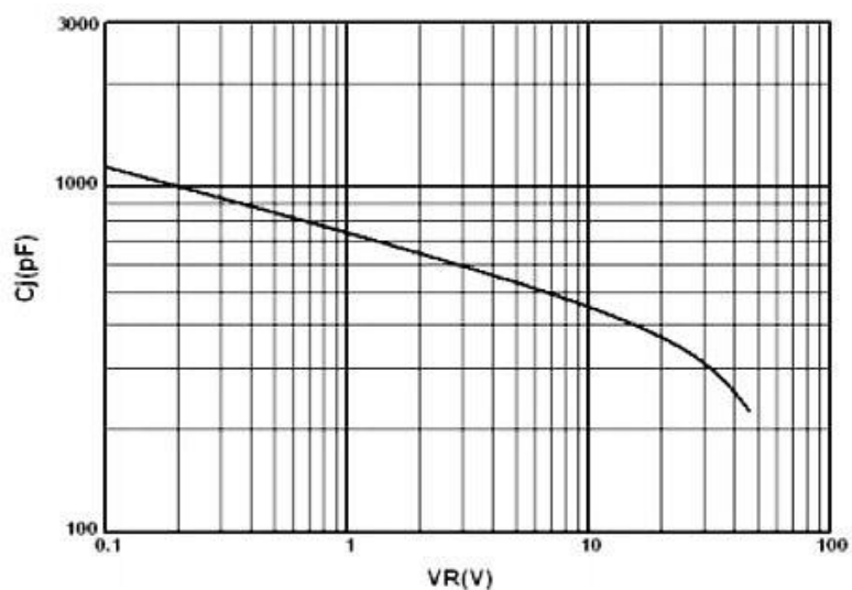
C_J vs V_R
