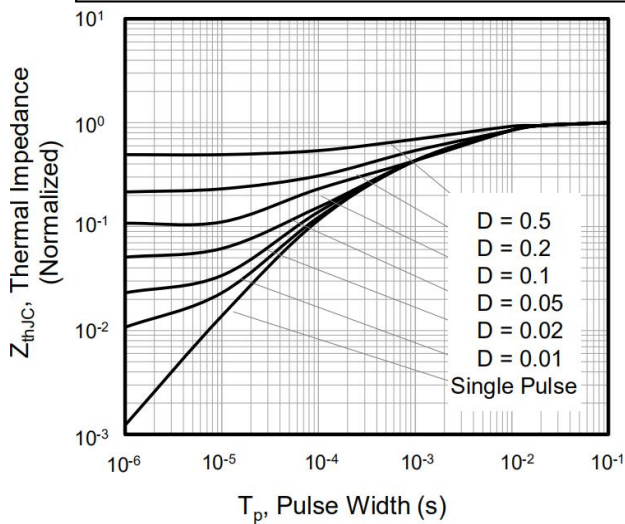
Transient Thermal Response Curve For MT40ND6A
