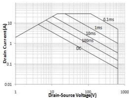
Maximum Safe Operating Area For MS65R280/TO-220MF-K1 /K4
