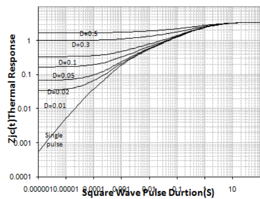
Transient Thermal Response Curve For MS65R280/TO-220MF-K1 /K4
