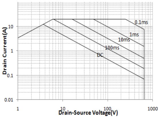
Maximum Safe Operating Area For MS65R190R/TO-247
