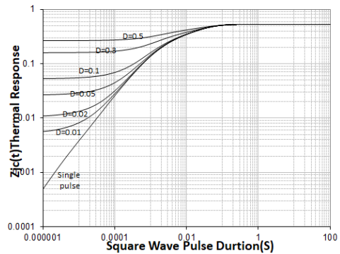
Transient Thermal Response Curve For MS65R190R/TO-247
