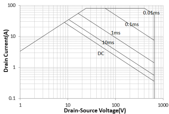
Maximum Safe Operating Area For MS65R190R/TO-247
