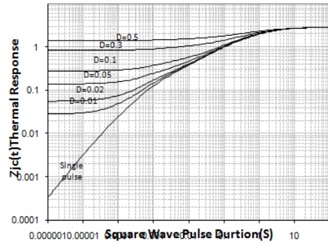
Transient Thermal Response Curve For MS65R190R/TO-220MF-K1
