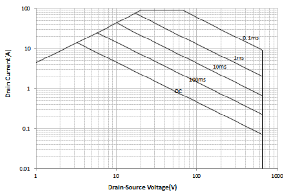
Maximum Safe Operating Area For MS65R135R/T0-247
