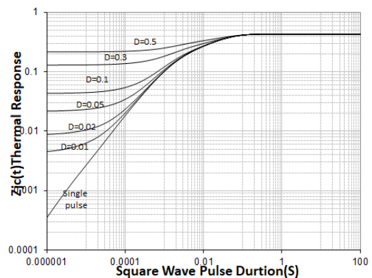
Transient Thermal Response Curve For MS65R135R/T0-247
