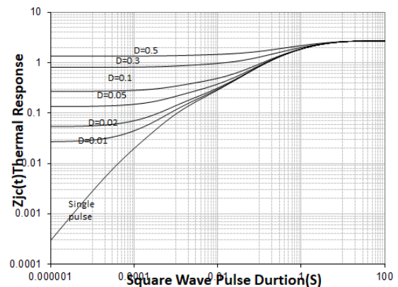
Transient Thermal Response Curve For MS65R135R/T0-247
