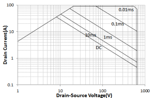
Maximum Safe Operating Area For MS65R135R/T0-247
