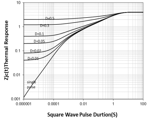
Transient Thermal Response Curve For MS60R650-TO-220MF
