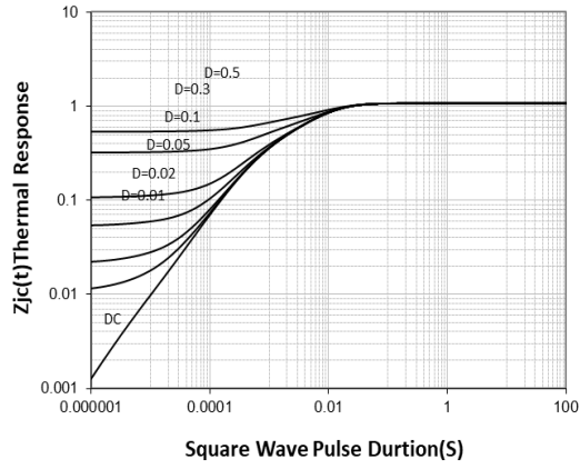
Transient Thermal Response Curve For MS60R650-DPAK
