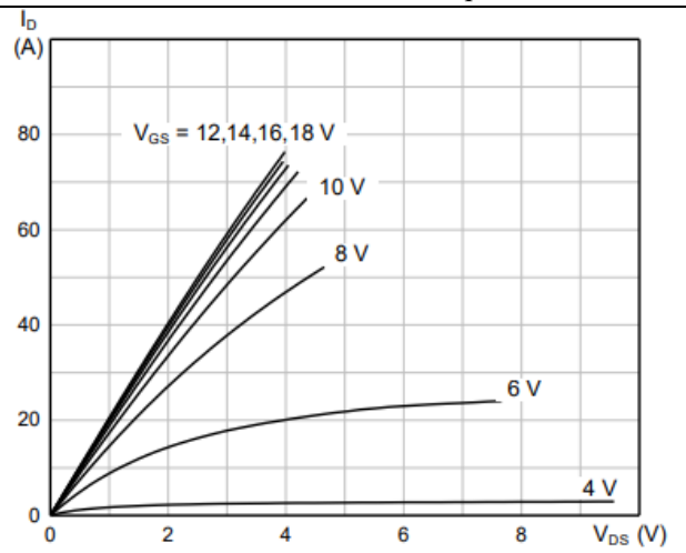
Output Characteristics T_J = 175\text{ }^{\circ}\text{C}
