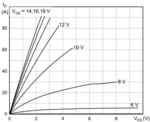
Output Characteristics T_J = 25\text{ }^{\circ}\text{C}
