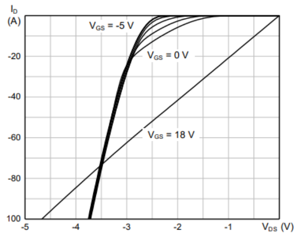
Body Diode Characteristics, T_J = 175\text{ }^{\circ}\text{C}
