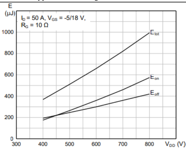
Typical Switching Energy vs. Supply Voltage
