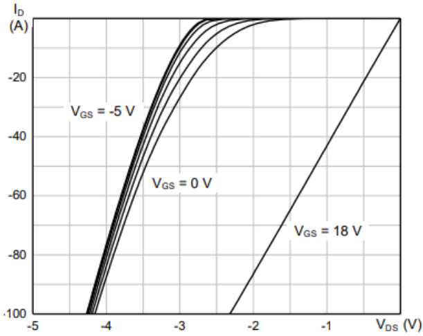
Body Diode Characteristics, T_J = 25\text{ }^{\circ}\text{C}
