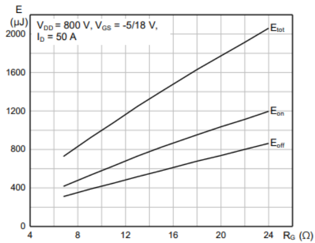
Typical Switching Energy vs. Gate Resistance
