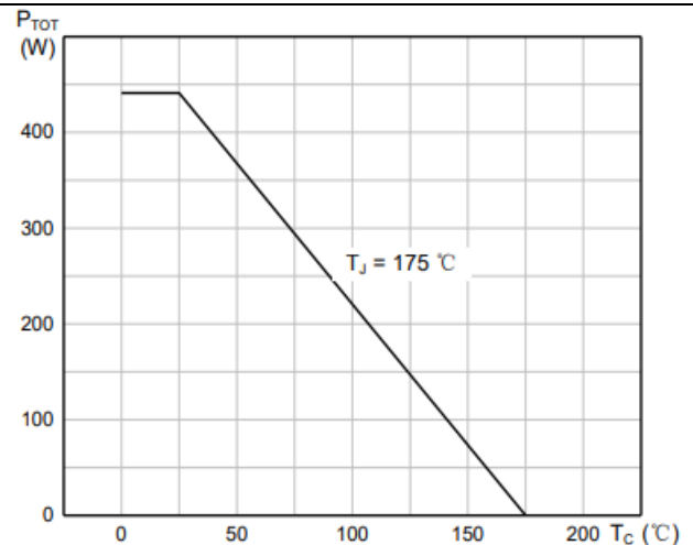
Total Power Dissipation
