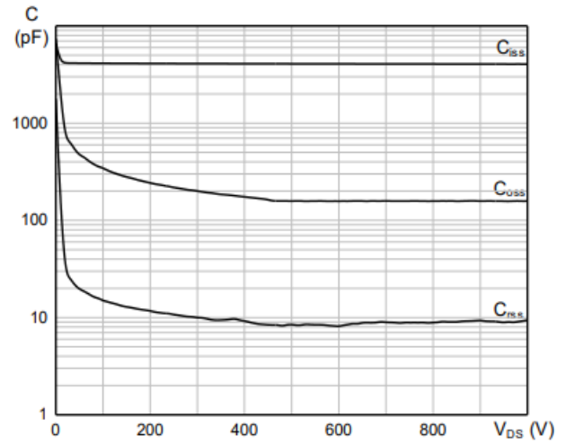
Typical Capacitance Characteristics
