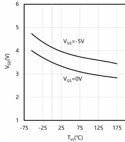
Typical reverse drain voltage as function of junction temperature V_{SD} = f(T_{VJ}) , I_{SD} = 2\text{ A}
