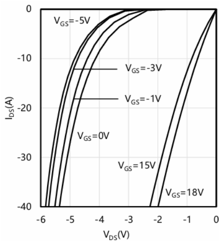
Typical reverse drain current as function of reverse drain voltage, V_{GS} as parameter I_{DS} = f(V_{DS}) , T_{VJ} = -55\text{ }^{\circ}\text{C}
