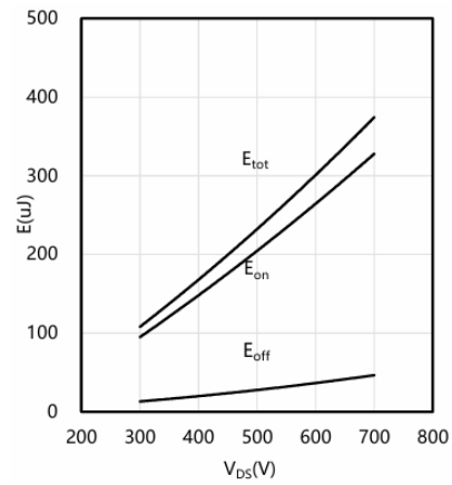
Typical switching energy losses as a function of V_{DS} , 2nd device own body diode T_{VJ} = 25\text{ }^{\circ}\text{C}
