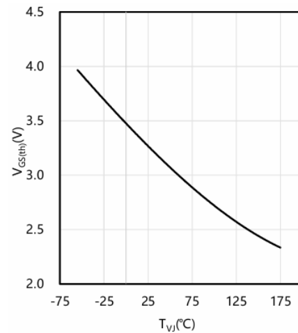
Typical gate-source threshold voltage as a function of junction temperature
