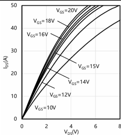
Typical output characteristic, V_{GS} as parameter T_{VJ} = 175\text{ }^{\circ}\text{C}
