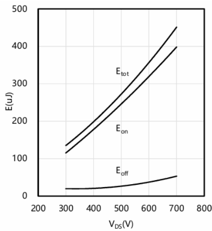
Typical switching energy losses as a function of V_{DS} , 2nd device own body diode T_{VJ} = 25\text{ }^{\circ}\text{C}
