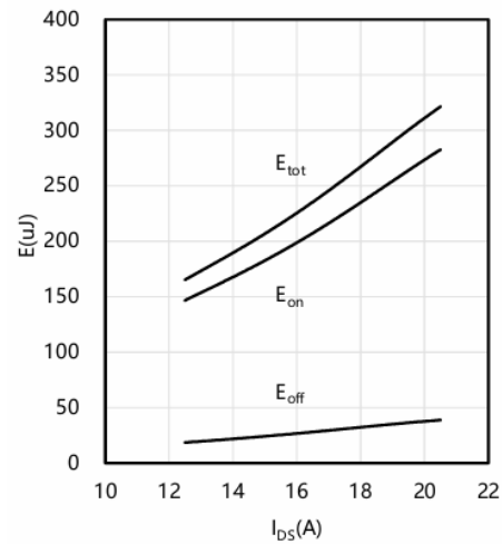
Typical switching energy losses as a function of I_{DS} , 2nd device own body diode T_{VJ} = 25\text{ °C}
