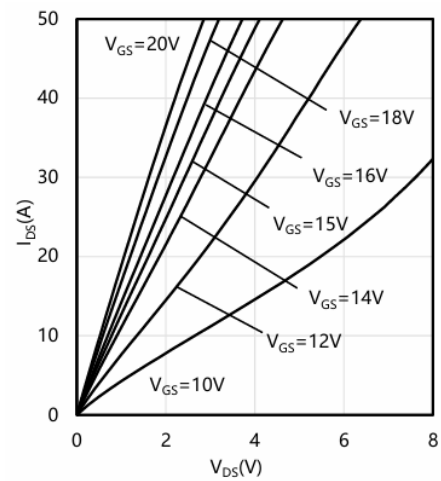
Typical output characteristic, V_{GS} as parameter T_{VJ} = 25\text{ }^{\circ}\text{C}
