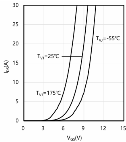
Typical transfer characteristic
