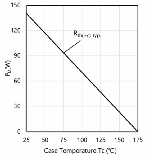
Power Derating
