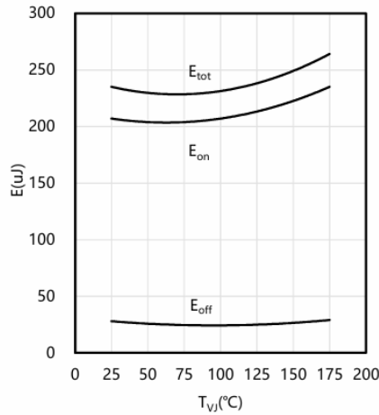
Typical switching energy as a function of junction temperature, 2nd device own body diode
