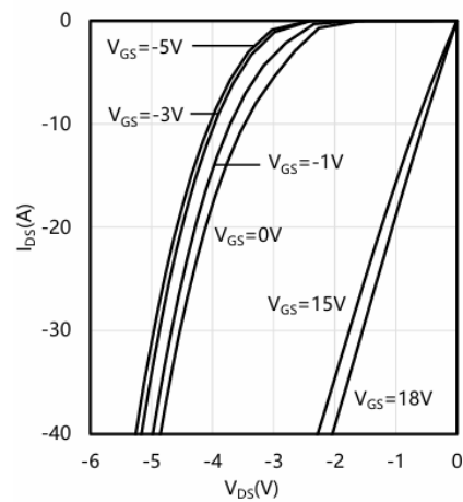
Typical reverse drain current as function of reverse drain voltage, V_{GS} as parameter I_{DS} = f(V_{DS}) , T_{VJ} = 25\text{ }^{\circ}\text{C}
