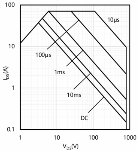
Safe operating area (SOA)
