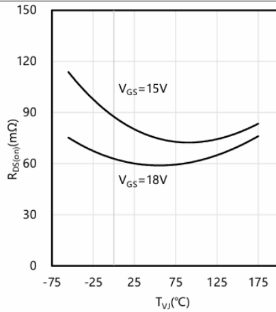
Typical on-state resistance as a function of temperature
