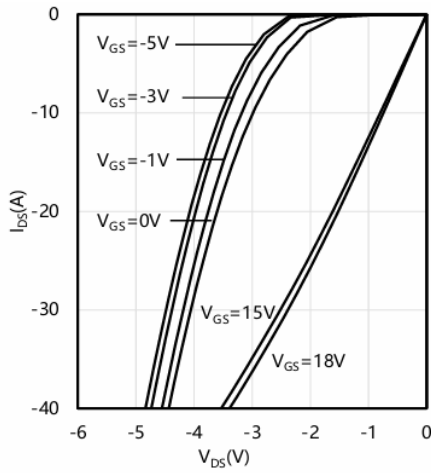
Typical reverse drain current as function of reverse drain voltage, VGS as parameter I_{DS} = f(V_{DS}) , T_{VJ} = 175\text{ °C}
