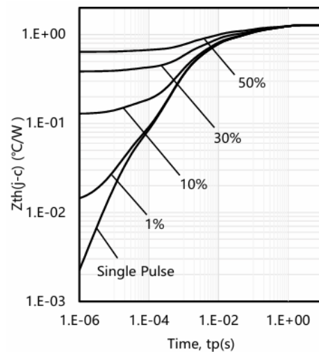
Transient thermal resistance (MOSFET)
