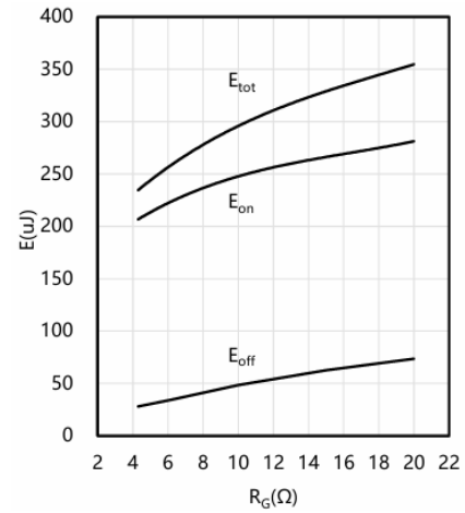
Typical switching energy losses as a function of gate resistance, 2nd device own body diode T_{VJ} = 25\text{ °C}
