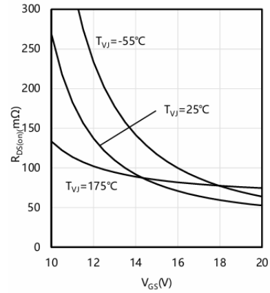
Typical on-state resistance as a function of V_{GS}
