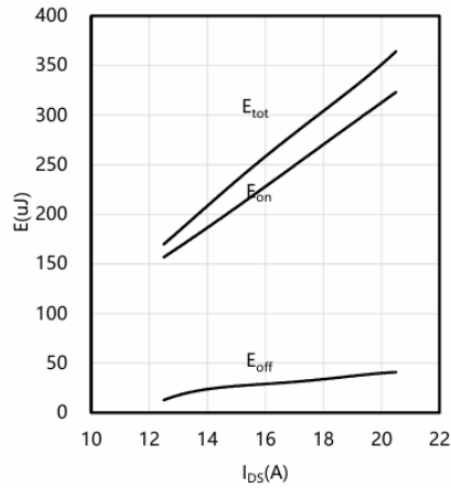
Typical switching energy losses as a function of I_{DS} , 2nd device own body diode T_{VJ} = 175\text{ }^{\circ}\text{C}
