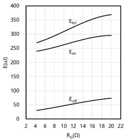
Typical switching energy losses as a function of gate resistance, 2nd device own body diode T_{VJ} = 175\text{ °C}
