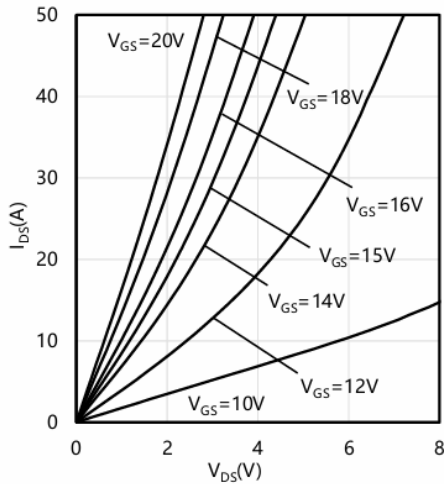
Typical output characteristic, V_{GS} as parameter T_{VJ} = -55\text{ }^{\circ}\text{C}
