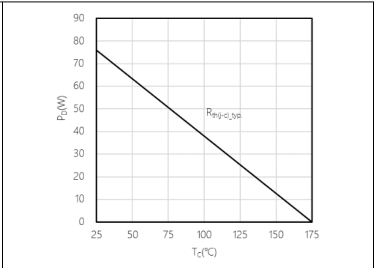
Power Derating
