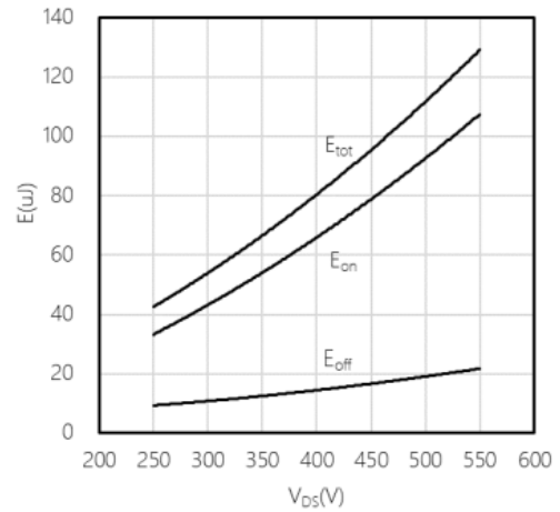
Typical switching energy losses as a function of V_{DS} , 2nd device own body diode T_{VJ} = 25\text{ °C}
