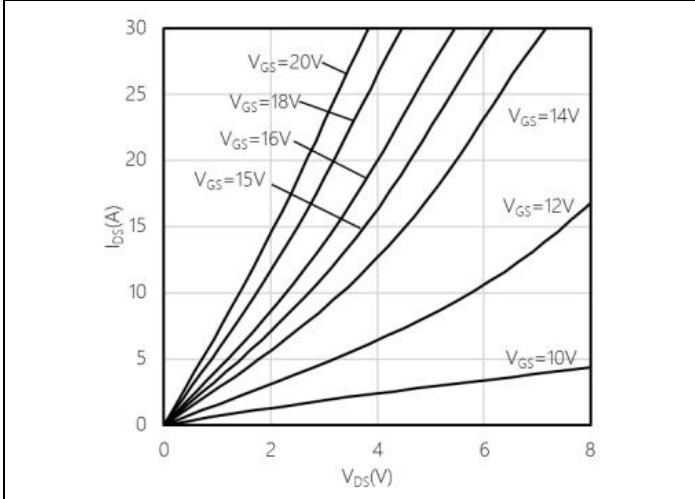
Typical output characteristic, V_{GS} as parameter T_{VJ} = -55^{\circ}\text{C}
