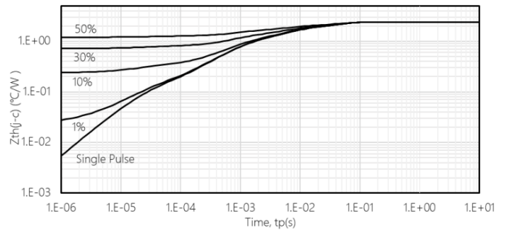
Transient thermal resistance (MOSFET)
