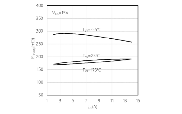
Typical on-state resistance as a function of drain current
