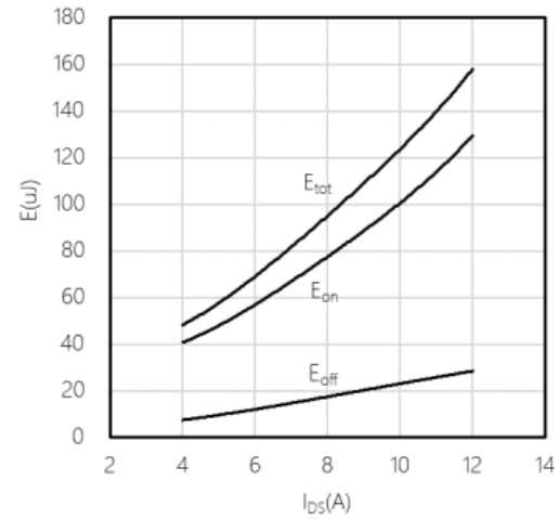
Typical switching energy losses as a function of I_{DS} , 2nd device own body diode T_{VJ} = 25\text{ °C}
