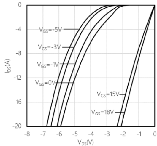
Typical reverse drain current as function of reverse drain voltage, V GS as parameter I_{DS} = f(V_{DS}), T_{VJ} = 25\text{ }^{\circ}\text{C}
