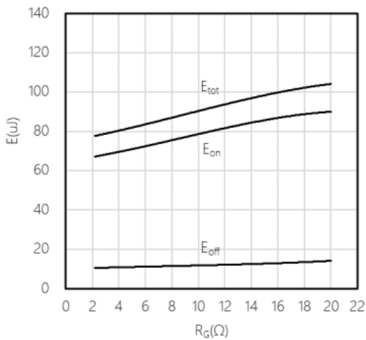
Typical switching energy losses as a function of gate resistance, 2nd device own body diode T_{VJ} = 175\text{ °C}
