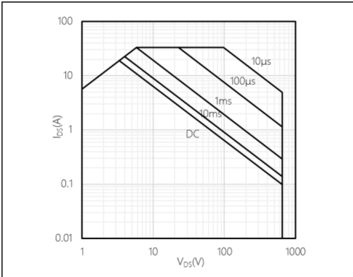
Safe operating area (SOA)
