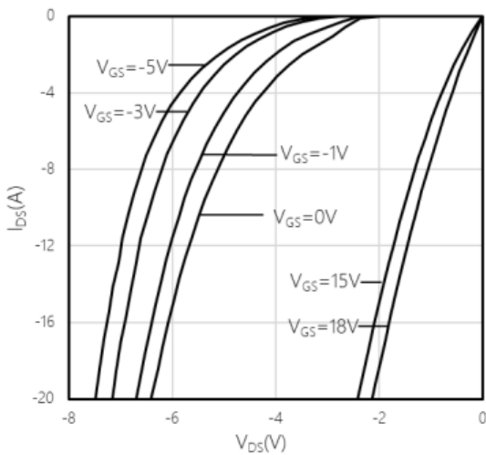
Typical reverse drain current as function of reverse drain voltage, V GS as parameter I_{DS} = f(V_{DS}), T_{VJ} = -55\text{ }^{\circ}\text{C}
