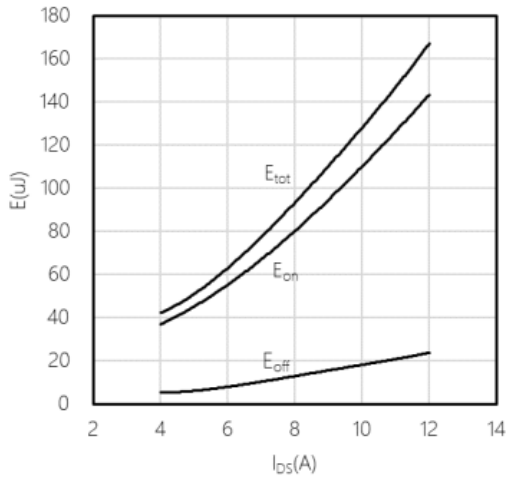
Typical switching energy losses as a function of I_{DS} , 2nd device own body diode T_{VJ} = 175\text{ °C}
