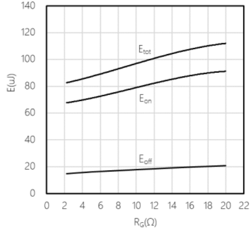
Typical switching energy losses as a function of gate resistance, 2nd device own body diode T_{VJ} = 25\text{ °C}
