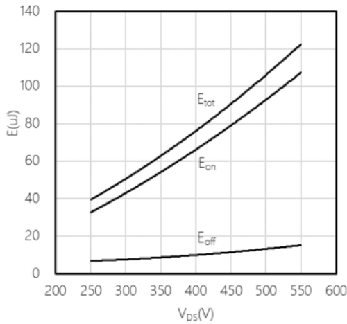
Typical switching energy losses as a function of V_{DS} , 2nd device own body diode T_{VJ} = 25\text{ °C}
