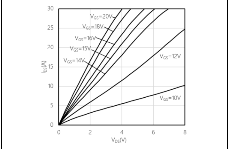
Typical output characteristic, V_{GS} as parameter T_{VJ} = 25^{\circ}\text{C}
