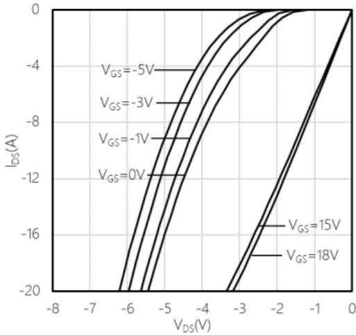
Typical reverse drain current as function of reverse drain voltage, VGS as parameter I_{DS} = f(V_{DS}), T_{VJ} = 175\text{ °C}
