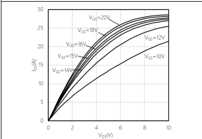
Typical output characteristic, V_{GS} as parameter T_{VJ} = 175^{\circ}\text{C}
