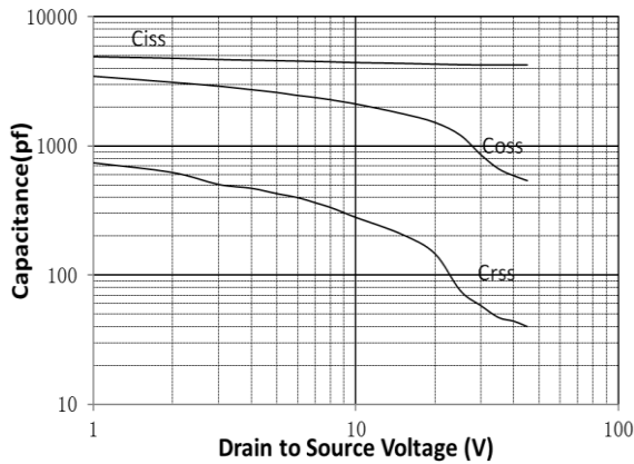
Capacitance Characteristics
