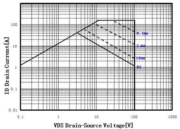
Maximum Safe Operation
