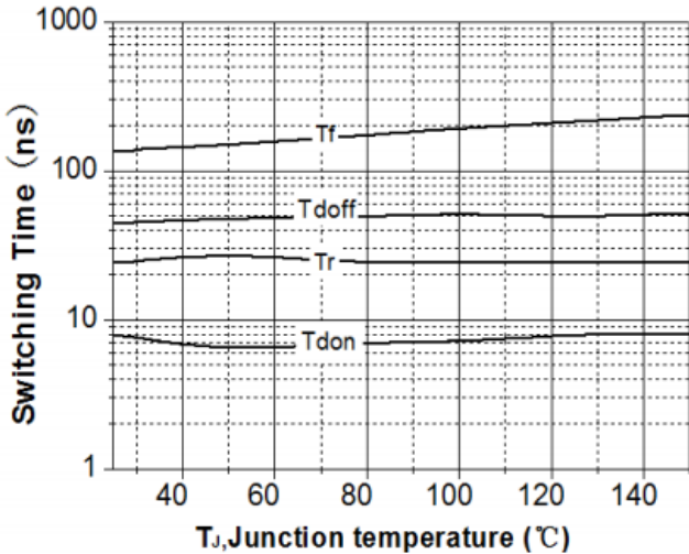
Switching Time vs Tj
