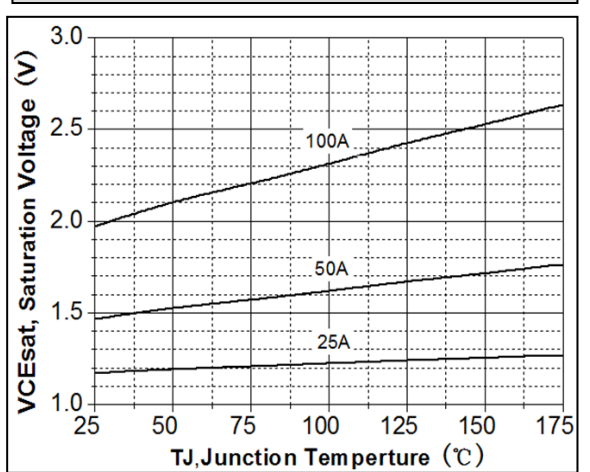
IGBT Vcesat vs. Tj
