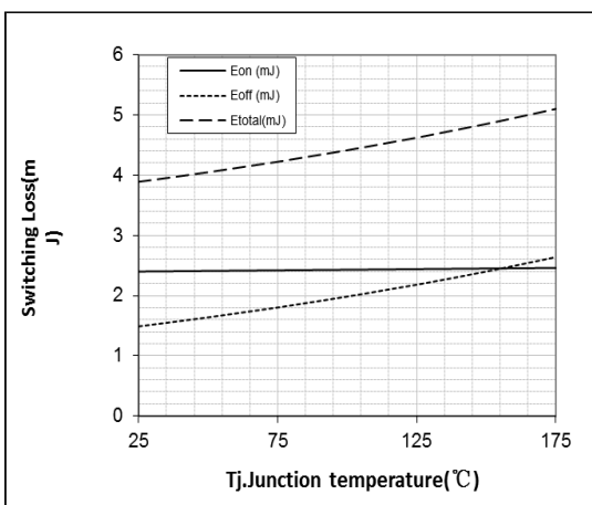
IGBT Switching Loss vs. T_j
