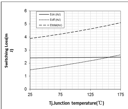
IGBT Switching Loss vs. T_j
