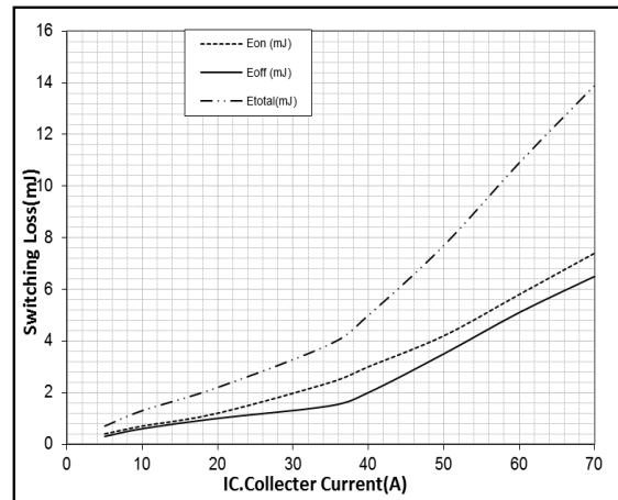
IGBT Switching Loss vs. I_c ( 25^{\circ}\text{C} )
