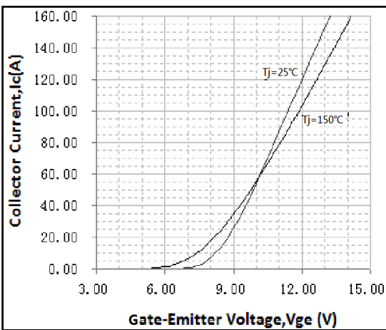
IGBT Transfer characteristic V_{CE}=20\text{V}
