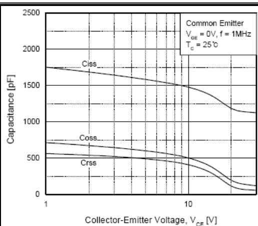
Capacitance Characteristics
