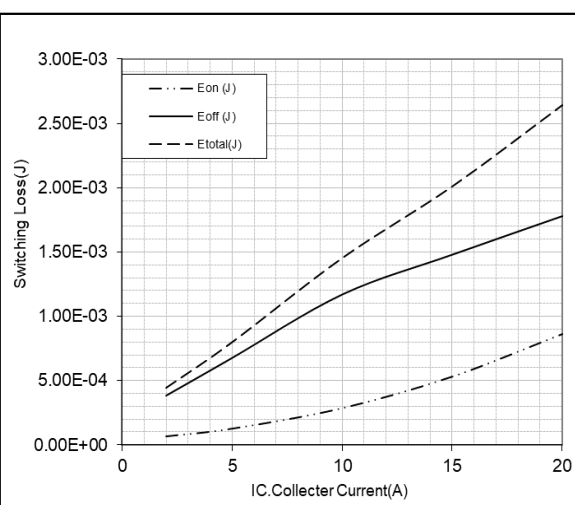
Inverter/Brake-Chopper IGBT Switching Loss vs. IC(25°C)
