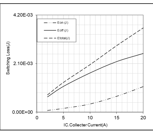
Inverter/Brake-Chopper IGBT Switching Loss vs. IC(175°C)
