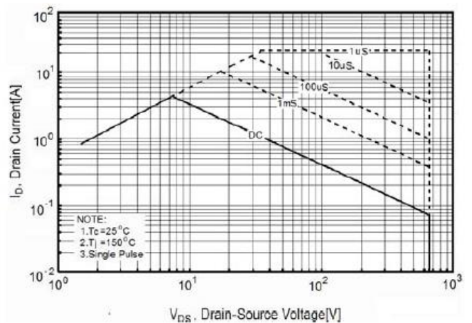
Maximum Safe Operating Area For JS70R700FU
