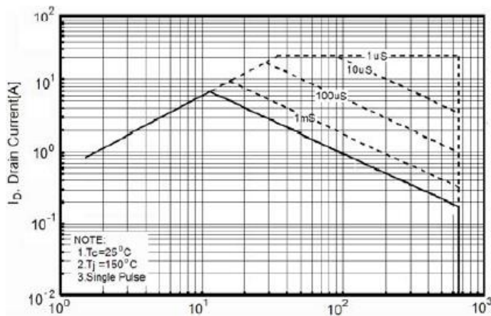
Maximum Safe Operating Area For JS65R600VU/RU/CU/SU
