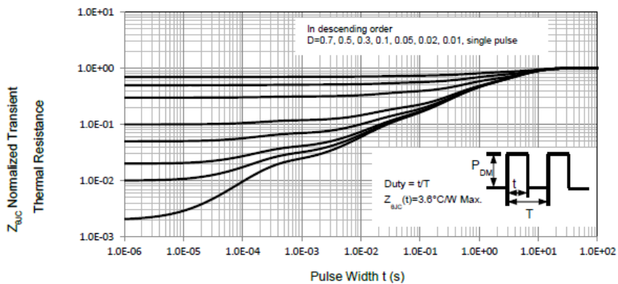
Transient Thermal Response Curve For JS65R190FU
