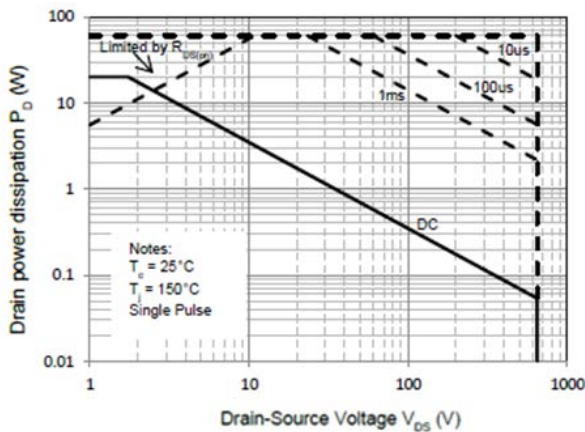
Maximum Safe Operating Area For JS65R190FU
