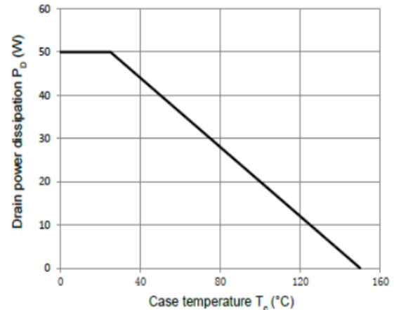
Power Dissipation vs. Temperature For JS60R900V/R/CU
