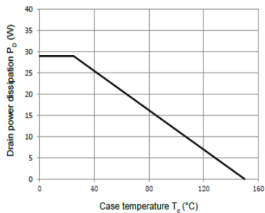
Power Dissipation vs. Temperature For JS60R900FU
